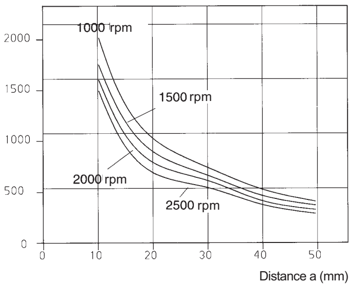
Radial loads (daN)
